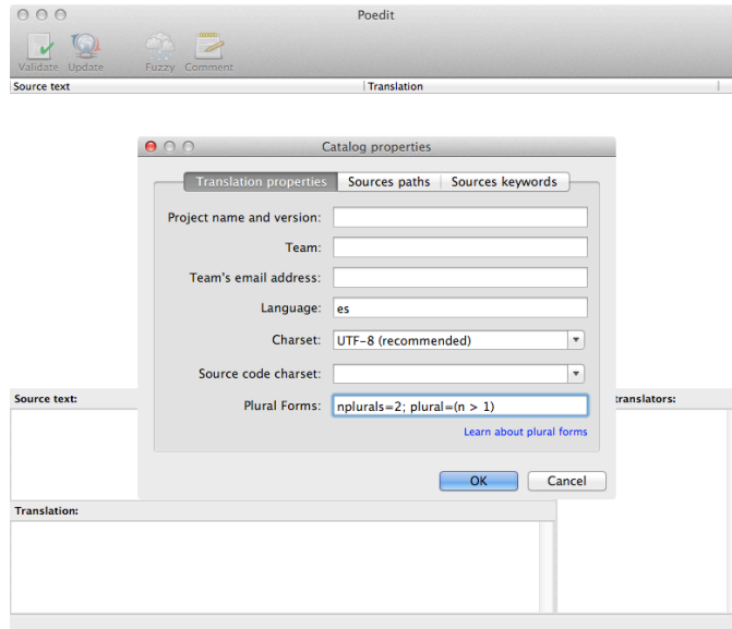
Setting plural forms
